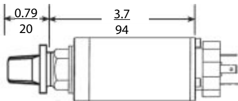
Shown w/DIN #43650 Electrical Connector and 1/4-18 NPT Male Pressure Fitting
