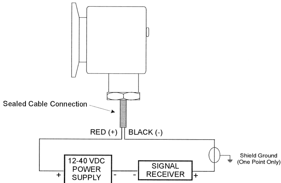
Figure 2 Wiring Diagram
