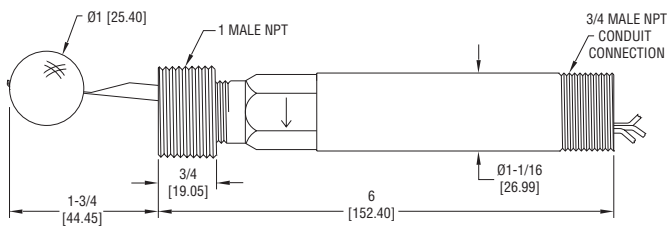
Polypropylene Float
