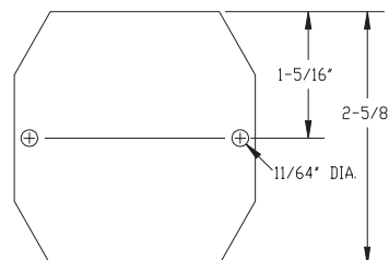
Relay Type 3 Dimensions
