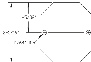
Relay Type 1 Dimensions
