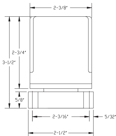
Relay Type 3 Dimensions
