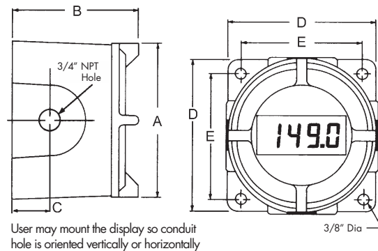
Figure 3. Mounting Dimensions
