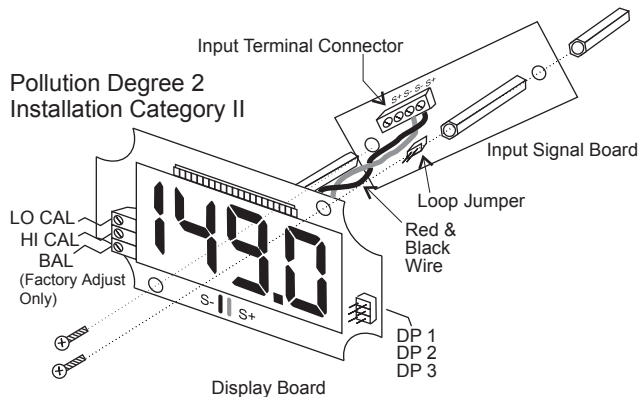
Figure 1. Assembly
